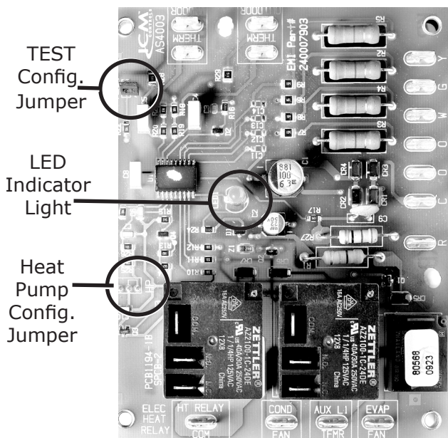
Figure 8 - Control Board
