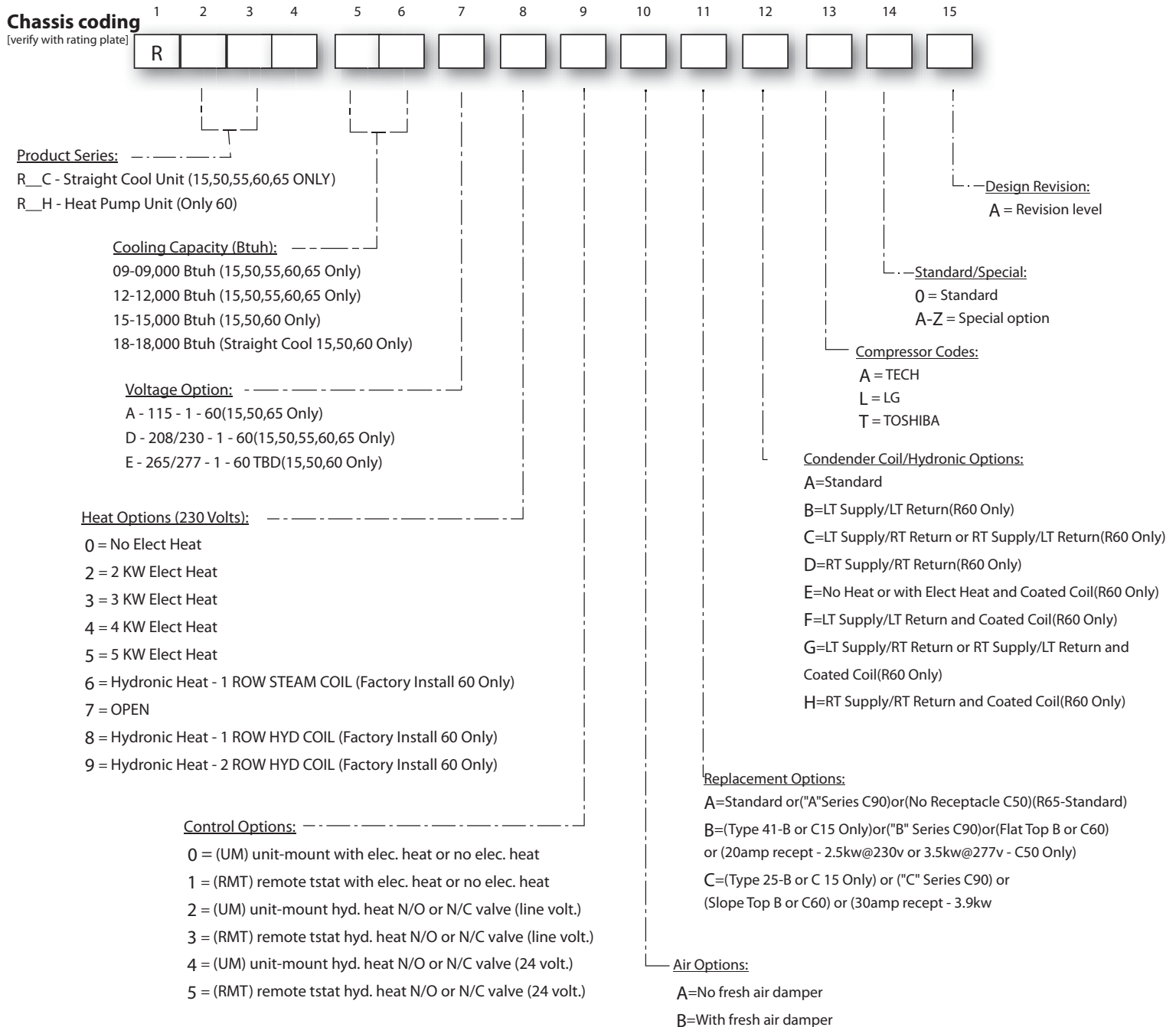
Figure 4 Model coding
