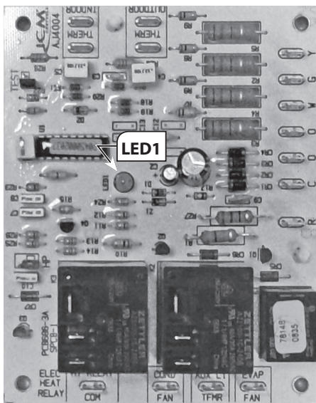
Figure 3 Indicator LED1
