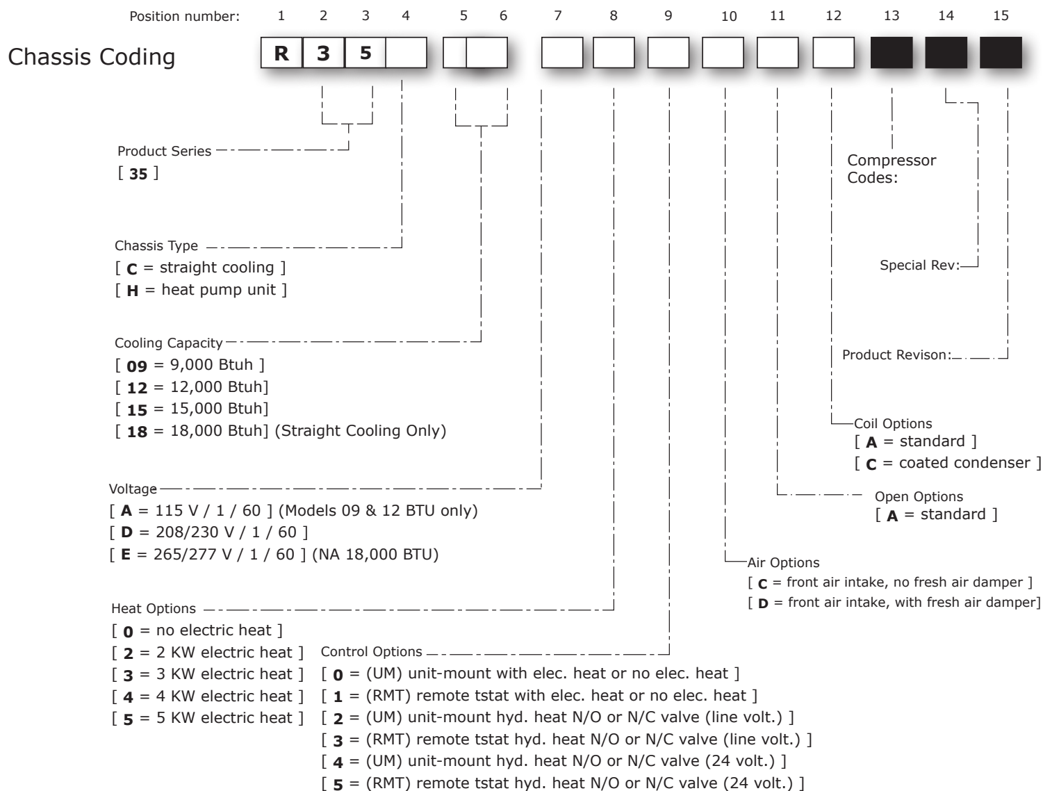
Figure 5 Model Coding
