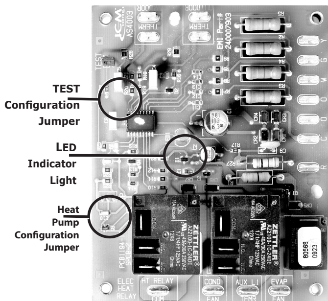
Figure 6 Control Board
