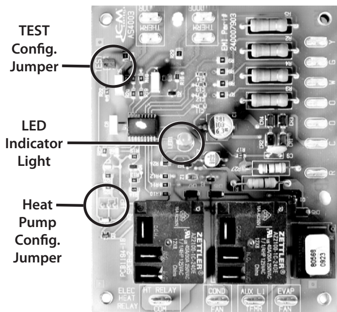
Figure 9 - Control Board
