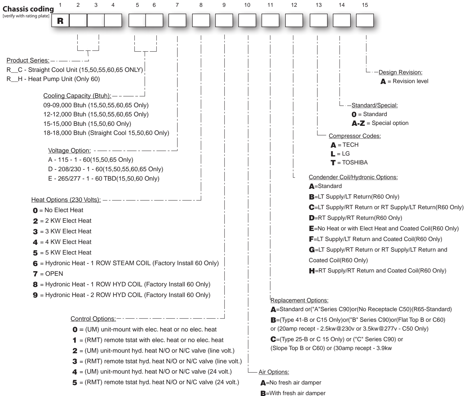
Figure 4 Model coding
