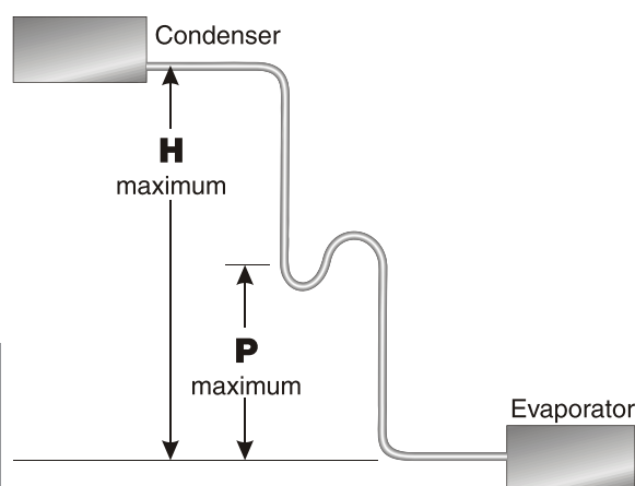
Figure 14 P-trap placement (see Table 1, Page 11 for dimensions H & P )
