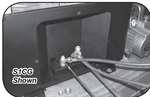
Figure 18 Manifold set connections at unit
