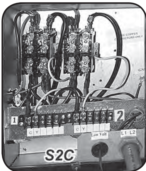
Figure 11 Completed wiring, S2CG
