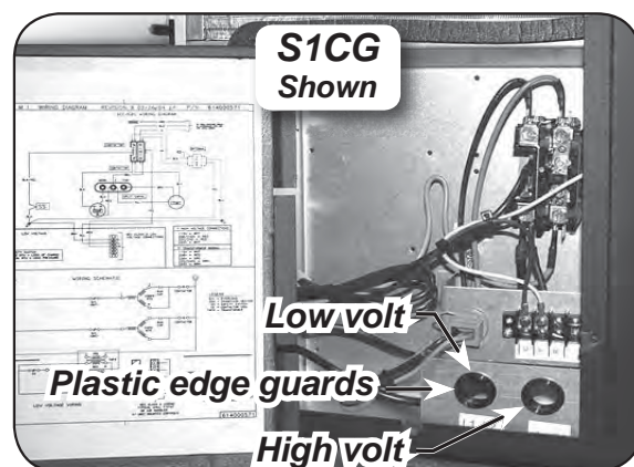
Figure 7 Power entrances
