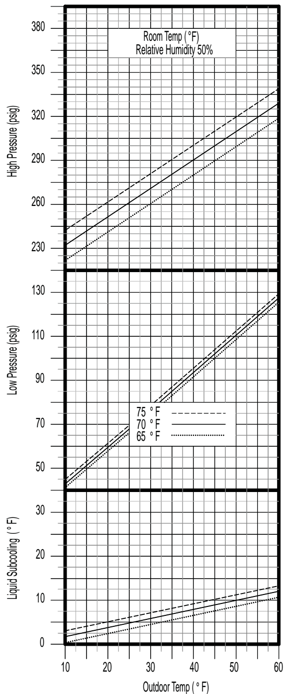
Model S1HG8000 with EMI's CAH24 (R-410A Ref.)
