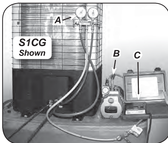
Figure 19 Manifold set up for evacuation
