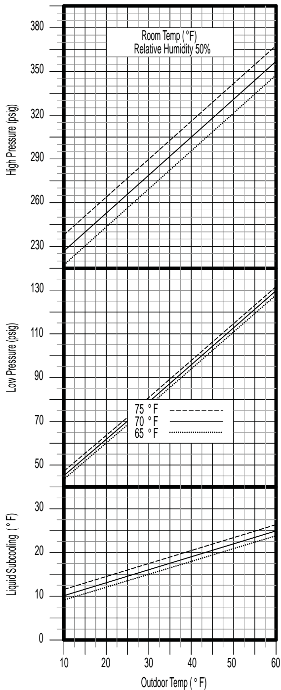
Model S1HG8000 with EMI's WLHG24 & UNHG24 (R-410A Ref.)
