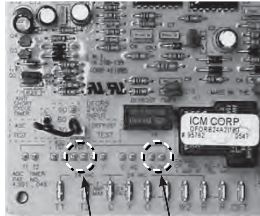
Figure 21 Defrost control board ( S1H shown )
