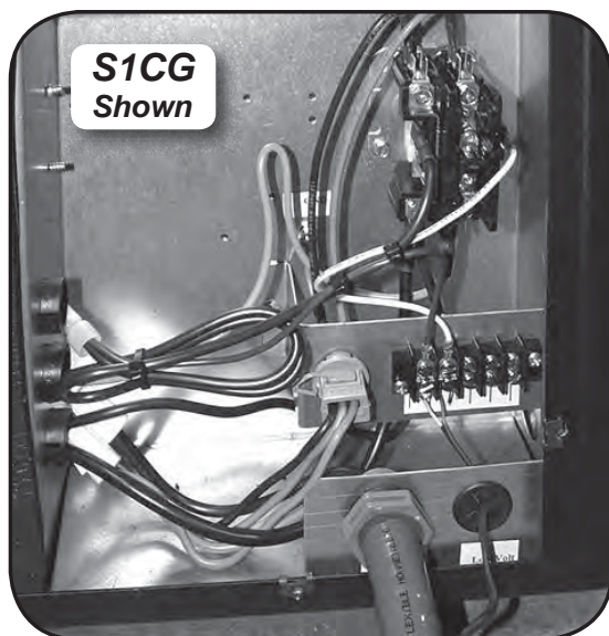
Figure 10 Completed wiring, S1CG
