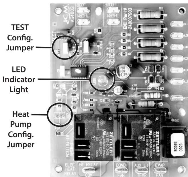
Figure 3 - Control Board
