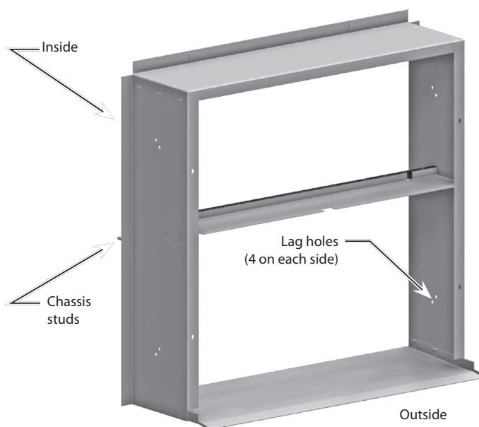
Figure 12 Typical tabbed-assembly wall sleeve (09–24)
