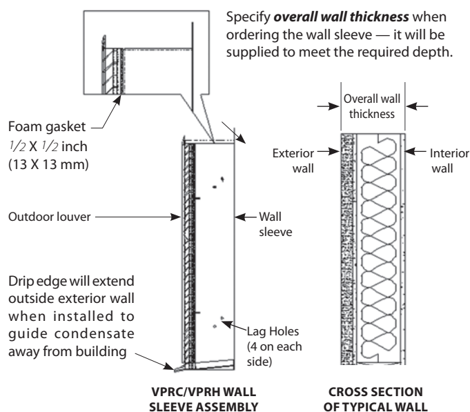
Figure 11 Determining wall sleeve depth
