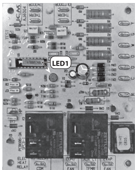
Figure 3 Indicator LED1
