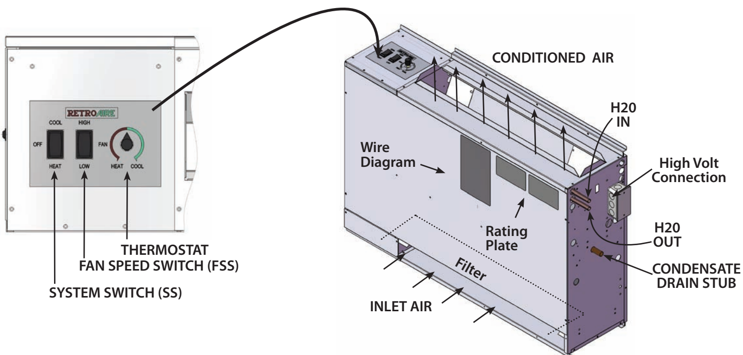
Figure 2 WM Chassis (Right)
