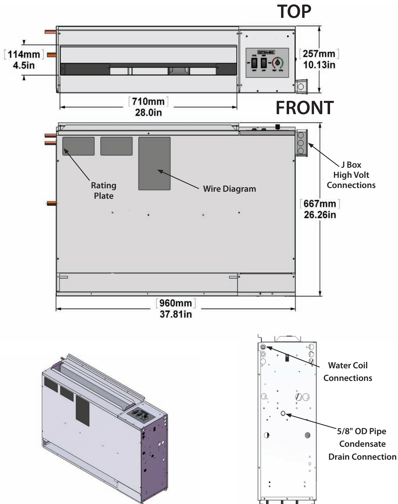
Figure 3 WM chassis
