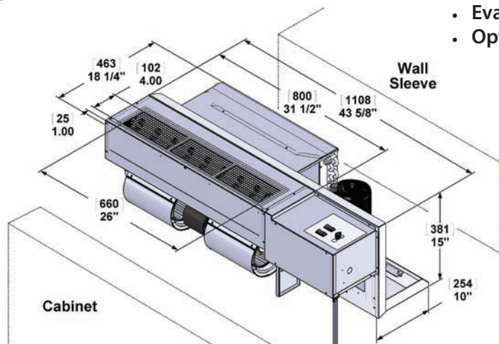
Figure 2 R35C | R35H chassis
