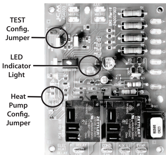
Figure 6 - Control Board
