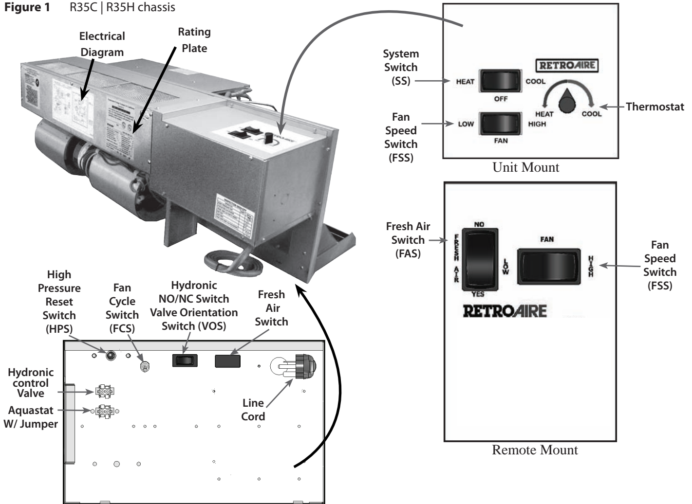
Figure 1 R35C | R35H chassis
