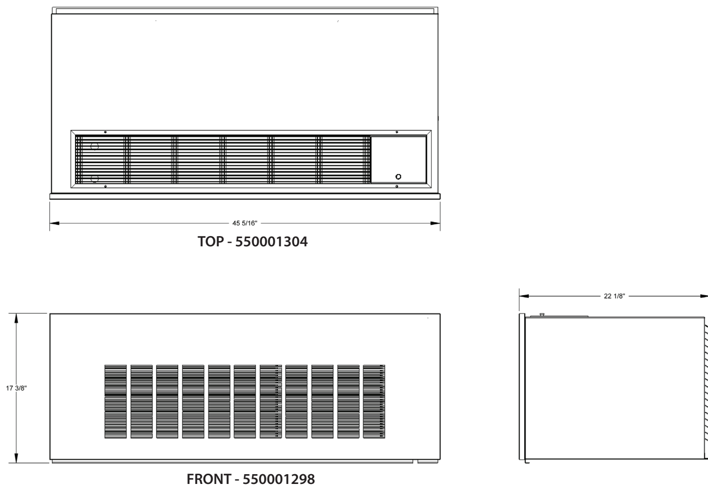
Figure 3 R35C | R35H Unit Cabinet and wall sleeve
