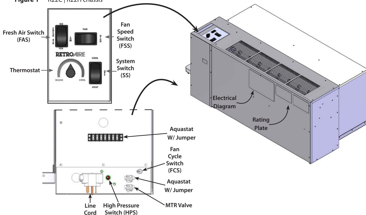
Figure 1 R22C | R22H chassis
