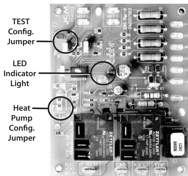
Figure 7 - Control Board
