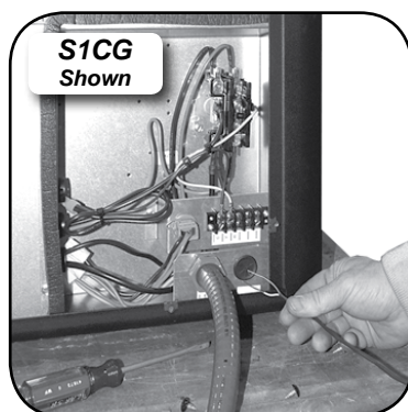
Figure 9 Low voltage connections
