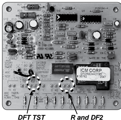
Figure 21 Defrost control board ( S1H shown )
