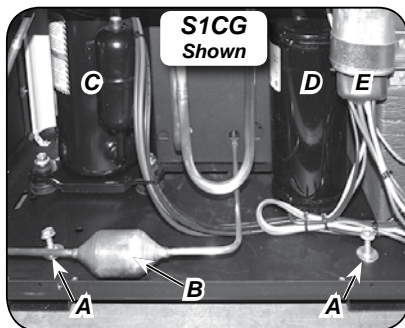
Figure 3 Bottom lag hole locations
