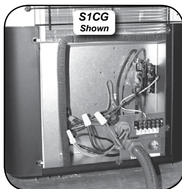
Figure 8 High voltage connections
