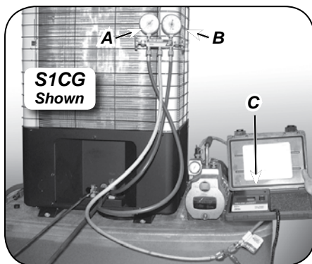
Figure 19 Manifold set up for evacuation
