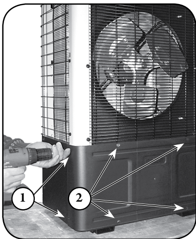
Figure 1 Remove front panel screws
