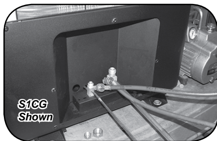
Figure 18 Manifold set connections at unit
