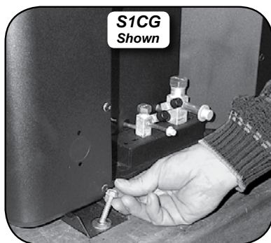
Figure 4 Lag holes in feet
