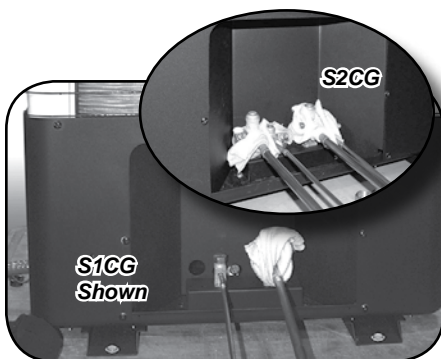
Figure 16 Wet rag “heat shield over valves
